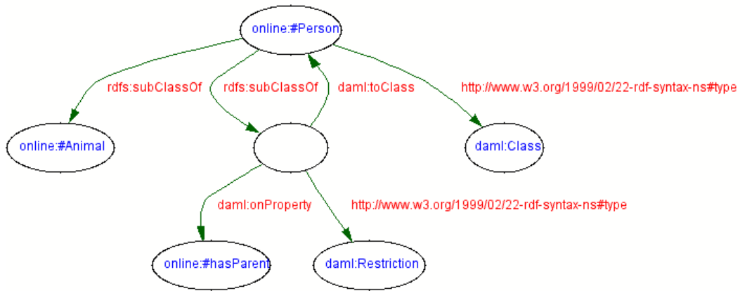
Figure 11: An RDF graph of a DAML class definition.
