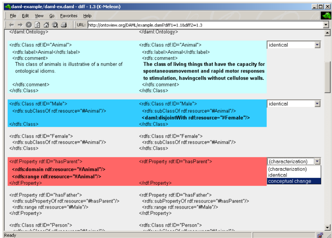
Figure 10: Comparing two ontologies
