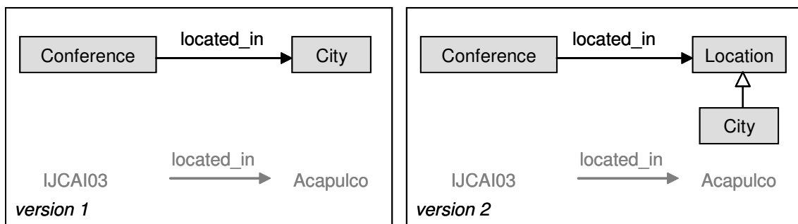
Figure 4: Two versions of a very simple ontology and a piece of associated data.
