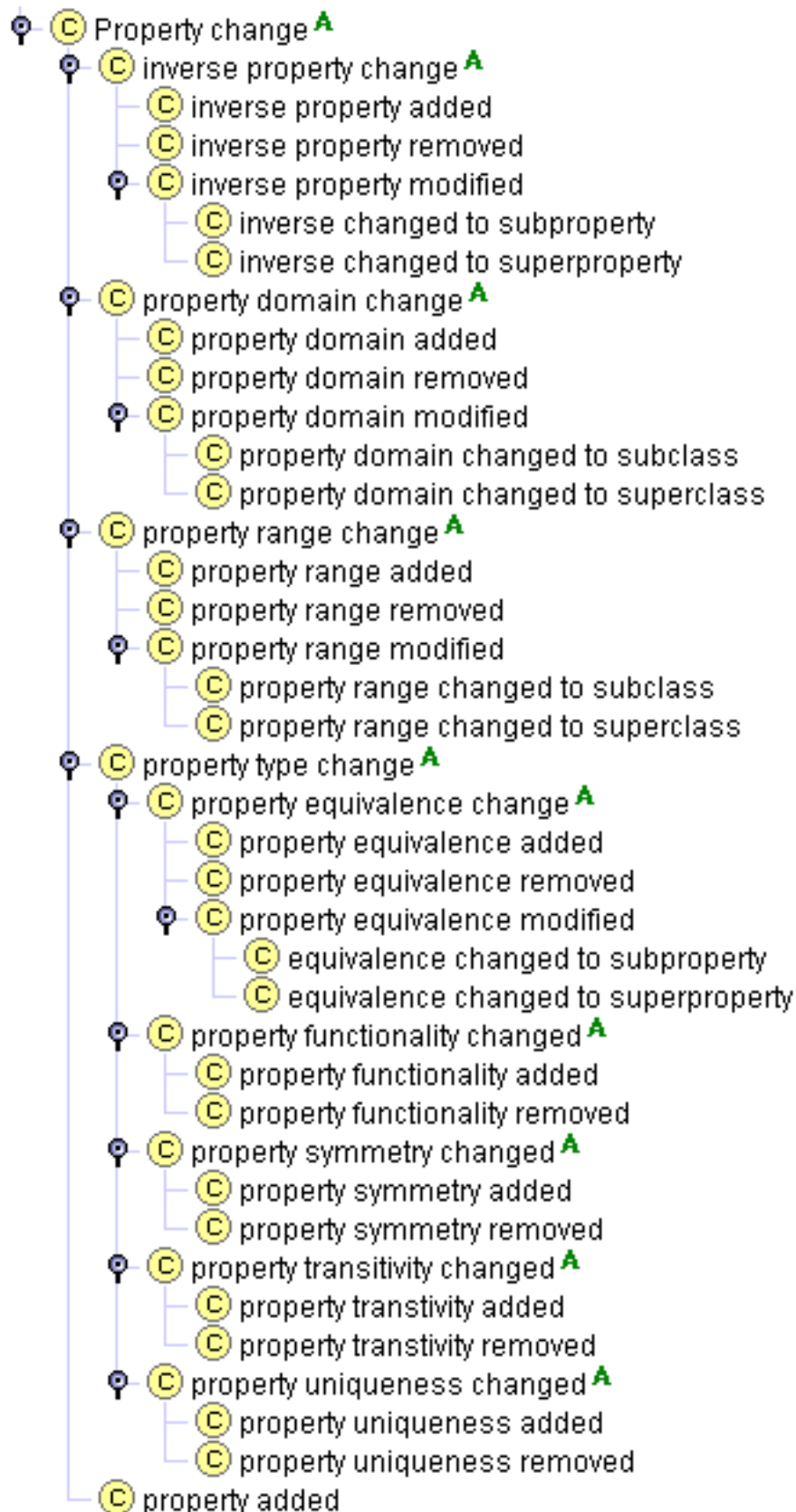
Figure 7: Possible changes in properties.
