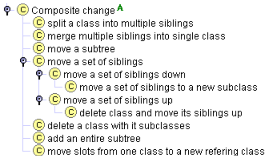
Figure 9: Some named composite changes.
