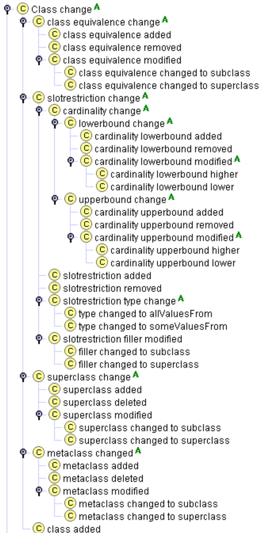
Figure 6: Possible changes in classes.
