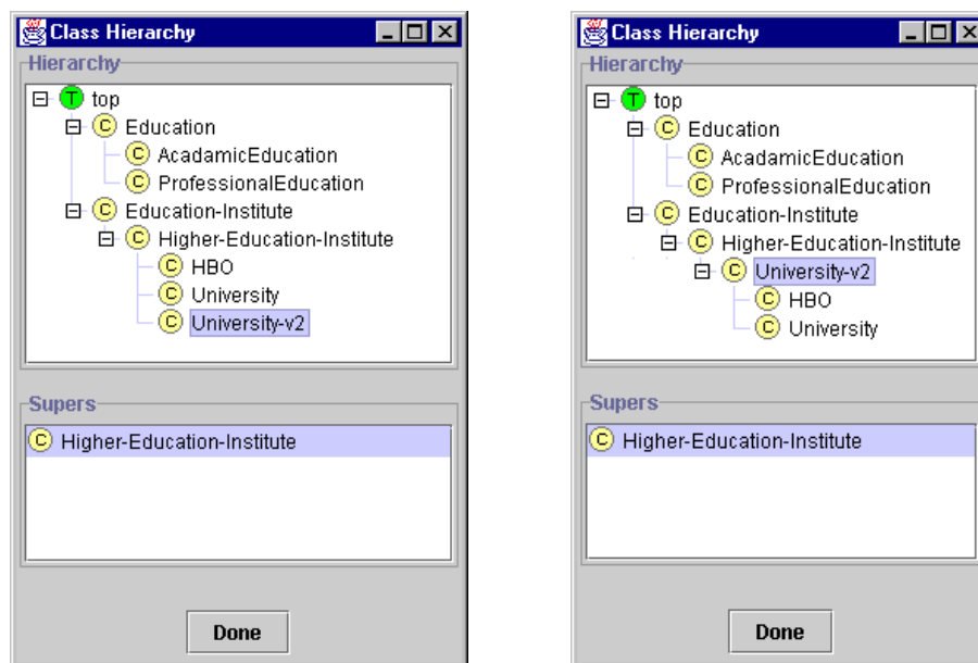
Figure 1: The hierarchy of the example ontology before and after classification with FaCT.
