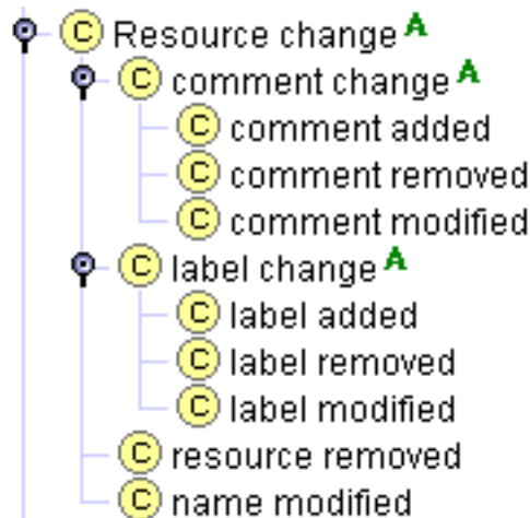
Figure 5: Possible changes of classes, properties, as well as instances.
